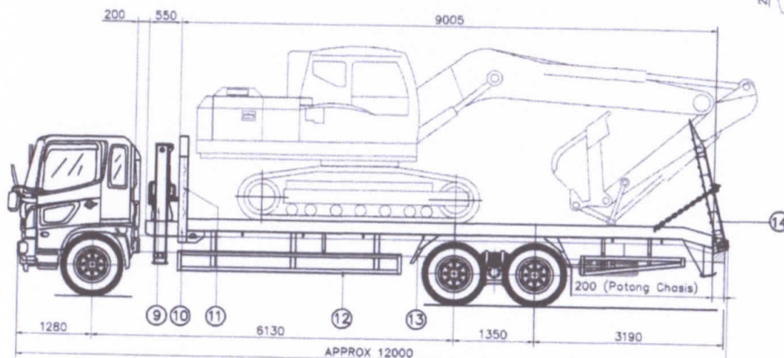
TAMPAK SAMPING
